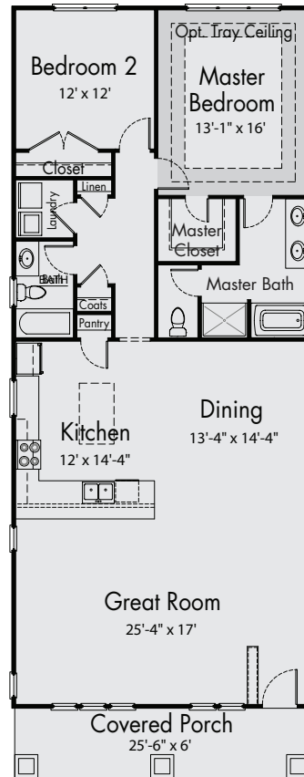
Opt. One-Level Plan, No Garage
